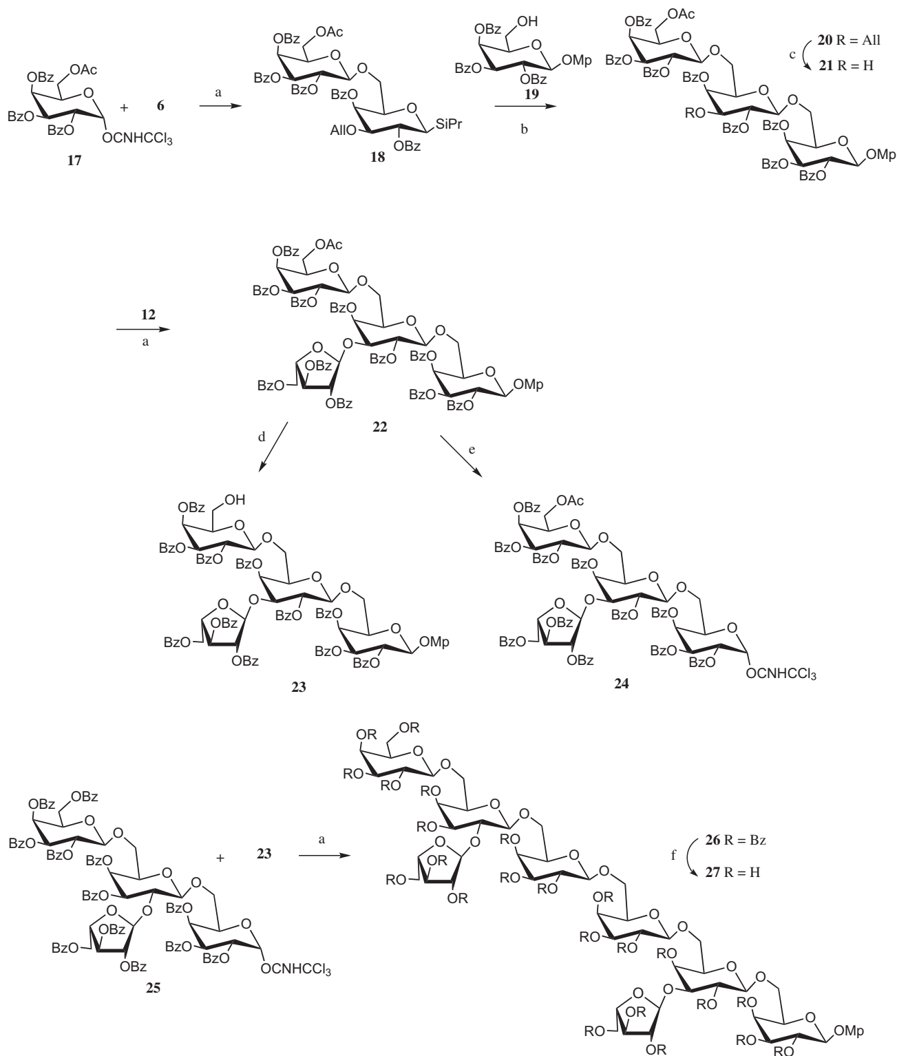
Scheme 2. Reagents and conditions: (a) TMSOTf, CH 2 Cl 2 , –20 °C to rt, 2–4 h; 83% for 18 , 81% for 26 . (b) TMSOTf (0.1–0.5 equiv), CH 2 Cl 2 , NIS (1.5 equiv), –20 °C to rt, 2–4 h; 90%. (c) PdCl 2 , CH 3 OH, 40 °C, 5 h, 94%. (d) 1:50:50 MeCOCl/CH 3 OH/CH 2 Cl 2 , rt, 48 h, 87%. (e) (i) CAN in MeCN–H 2 O, rt, 0.5 h; (ii) CH 2 Cl 2 , CCl 3 CN, K 2 CO 3 , rt, 10 h. (f) satd NH 3 /MeOH, rt, 7 d, 85%.
