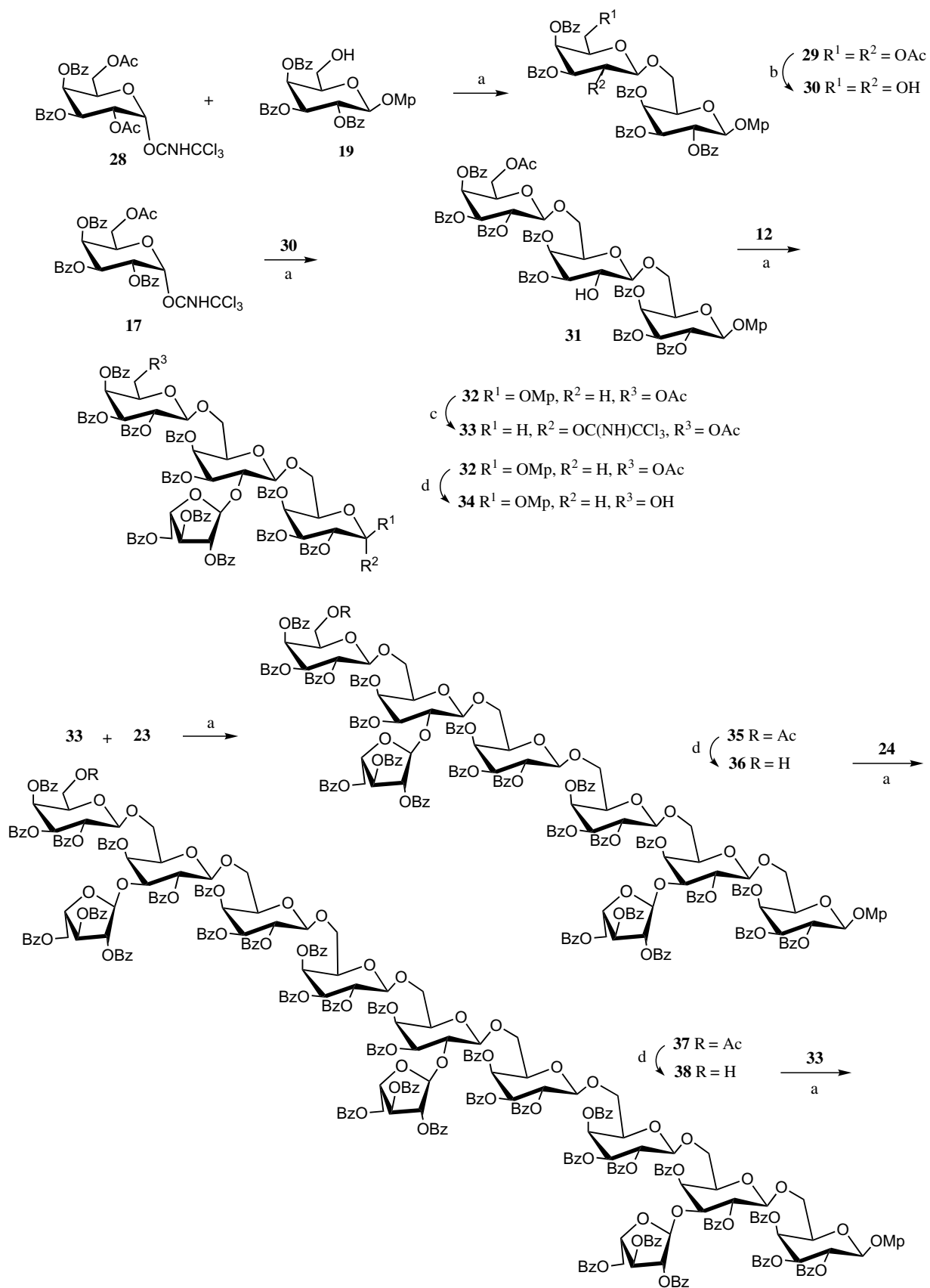
Scheme 3. Reagents and conditions: (a) TMSOTf, \text{CH}_2\text{Cl}_2 , -20^\circ\text{C} to rt, 2–4h; 89% for 29 , 81% for 31 , 89% for 32 , 81% for 35 , 75% for 37 , 71% for 39 , 65% for 41 , 81% for 43 . (b) 3:50:50 \text{MeCOCl}/\text{CH}_3\text{OH}/\text{CH}_2\text{Cl}_2 , rt, 48h, 71%. (c) (i) CAN in \text{MeCN}-\text{H}_2\text{O} , rt, 0.5h; (ii) \text{CH}_2\text{Cl}_2 , \text{CCl}_3\text{CN} , \text{K}_2\text{CO}_3 , rt, 10h. (d) 1:50:50 \text{MeCOCl}/\text{CH}_3\text{OH}/\text{CH}_2\text{Cl}_2 , rt, 48h; 83% for 34 , 81% for 36 , 71% for 38 , 71% for 40 . (e) satd \text{NH}_3/\text{MeOH} , rt, 7d, 85%.
