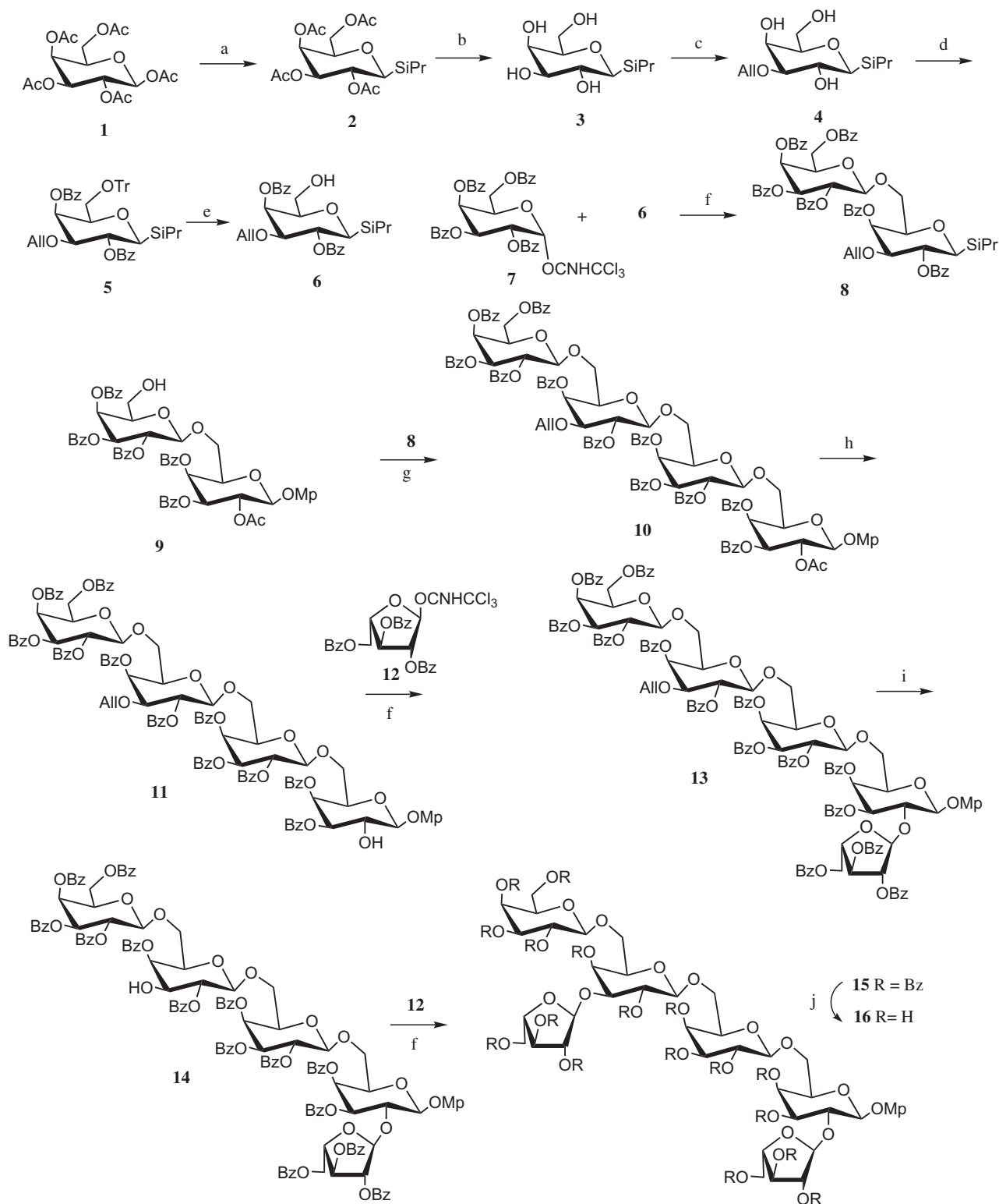
Scheme 1. Reagents and conditions: (a) CH 2 Cl 2 , i PrSH, Et 2 O·BF 3 , rt, 1.5 h, 75%. (b) CH 3 OH/CH 3 ONa, pH 10, rt, 5 h, 81%. (c) CH 3 OH, Bu 2 SnO, reflux 2 h, then AllBr, Bu 4 NI, toluene, 60 °C, 24 h, 79%. (d) Trityl chloride, (1.1 equiv), pyridine, 50 °C, 24 h, then PhCOCl, (2.4 equiv), 50 °C, overnight, 71%. (e) 1:500:500 MeCOCl/CH 3 OH/CH 2 Cl 2 , rt, 3 h, 80%. (f) TMSOTf, CH 2 Cl 2 , –20 °C to rt, 2–4 h; 85% for 8 , 87% for 13 , 89% for 15 . (g) TMSOTf (0.1–0.5 equiv), CH 2 Cl 2 , NIS (1.5 equiv), –20 °C to rt, 2–4 h; 92%. (h) 3:50:50 MeCOCl/CH 3 OH/CH 2 Cl 2 , rt, 48 h, 78%. (i) PdCl 2 , CH 3 OH, 40 °C, 5 h, 90% (j) satd NH 3 /MeOH, rt, 7 d, 90%.
